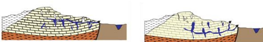
Figure 2: Left: Jurassien-type karst system with conduit networks close to the spring altitude. Right: Vauclusien-type karst system with conduit network developed below the spring. Figure modified after Marsaud (1997).
