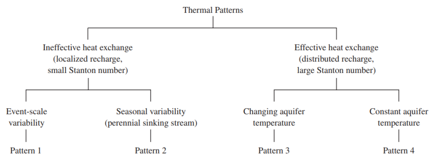
Figure 19 : Flow chart summary and patterns for heat transport in karst springs (Luhmann et al. 2011).
