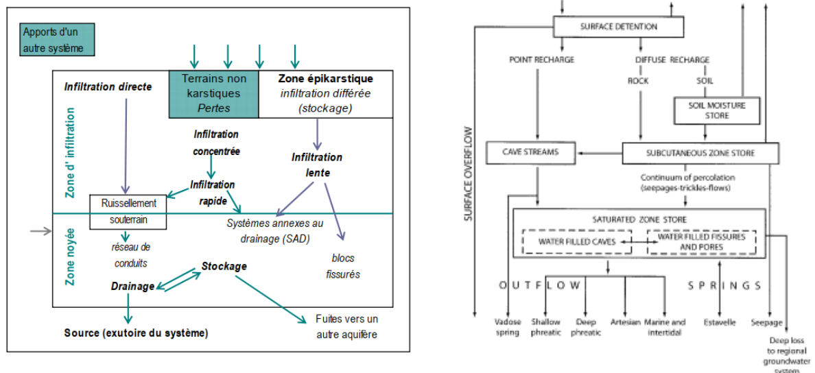
Figure 6: Conceptual models of karst system functioning accounting for flow, storage and recharge processes. Functioning diagram on the left and right from Mangin (1975) and Ford and Williams (2007) respectively
